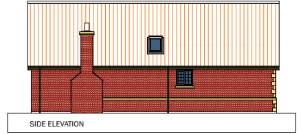
SIDE ELEVATION
